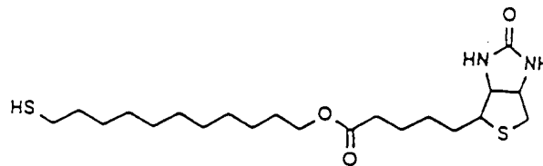
biotin compound 2
